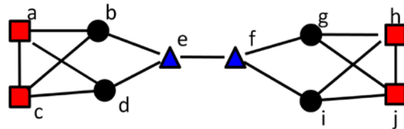
Figure 8. Shapes identify nodes that are structurally isomorphic.
