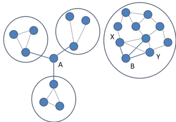
Figure 4. Node A has more structural holes than B
